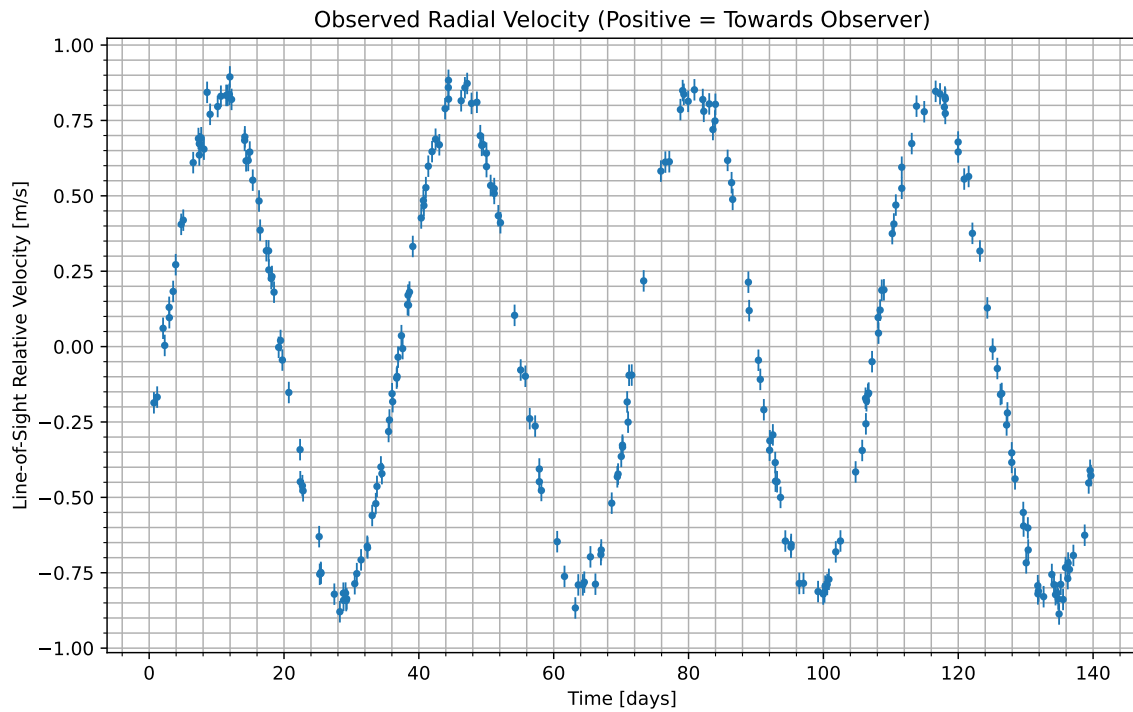
Figure 1: We have isolated the radial velocity of the host star due to the candidate planet. Data begins at UTC 2100-04-10/06:44. Positive values indicate the velocity at which the star is moving towards us; negative indicate the velocity at which it is moving away.
