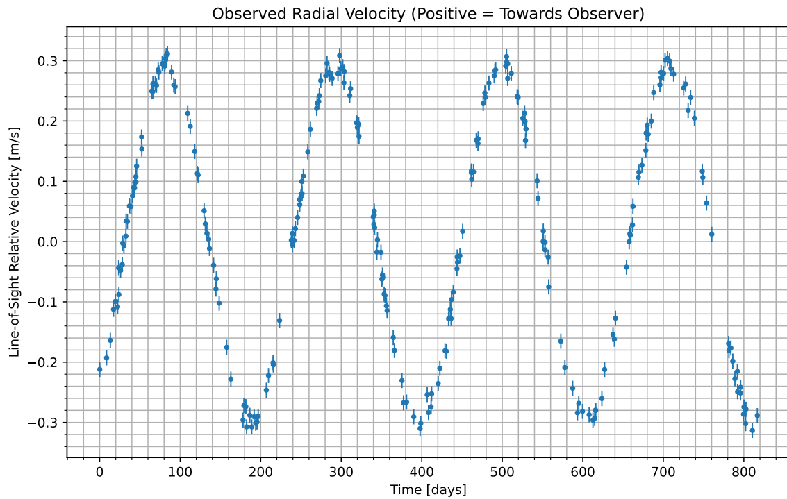
Figure 1: We have isolated the radial velocity of the host star due to the candidate planet. Data begins at UTC 2084-04-01/11:07. Positive values indicate the velocity at which the star is moving towards us; negative indicate the velocity at which it is moving away.
