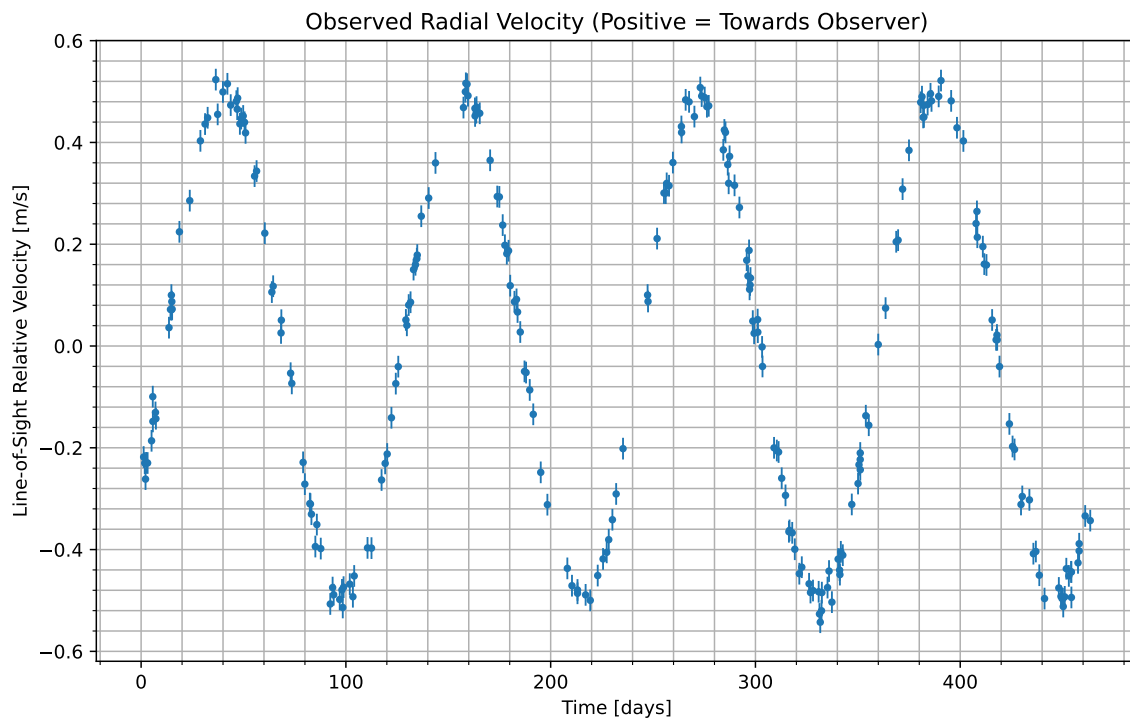
Figure 1: We have isolated the radial velocity of the host star due to the candidate planet. Data begins at UTC 2088-07-10/21:26. Positive values indicate the velocity at which the star is moving towards us; negative indicate the velocity at which it is moving away.
