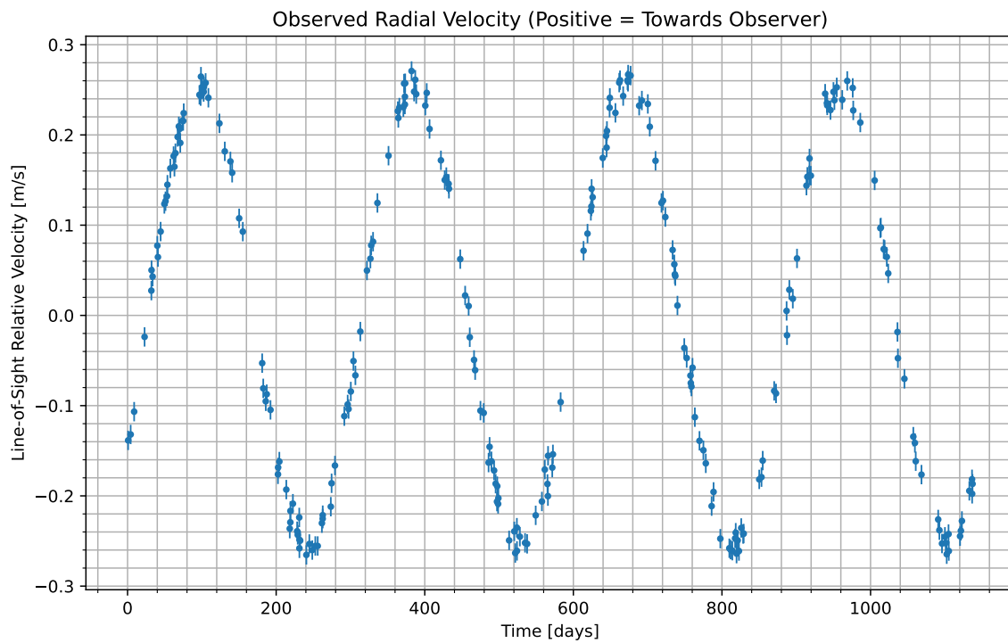
Figure 1: We have isolated the radial velocity of the host star due to the candidate planet. Data begins at UTC 2070-02-16/18:54. Positive values indicate the velocity at which the star is moving towards us; negative indicate the velocity at which it is moving away.
