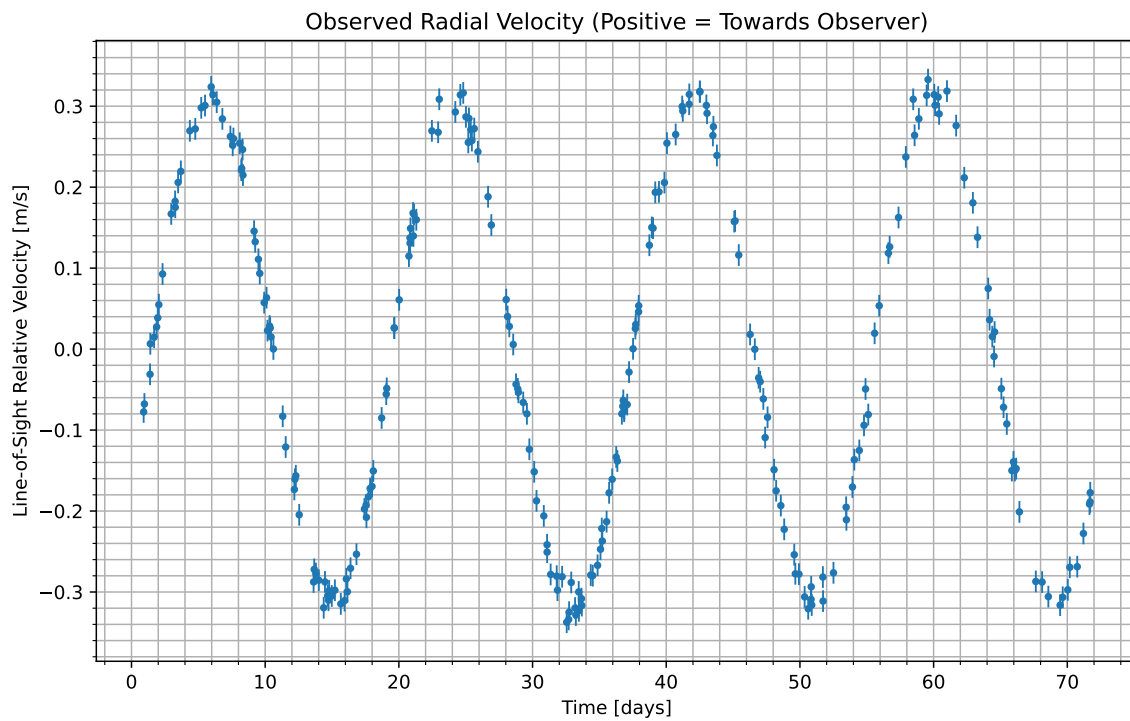
Figure 1: We have isolated the radial velocity of the host star due to the candidate planet. Data begins at UTC 2093-03-17/21:40. Positive values indicate the velocity at which the star is moving towards us; negative indicate the velocity at which it is moving away.
