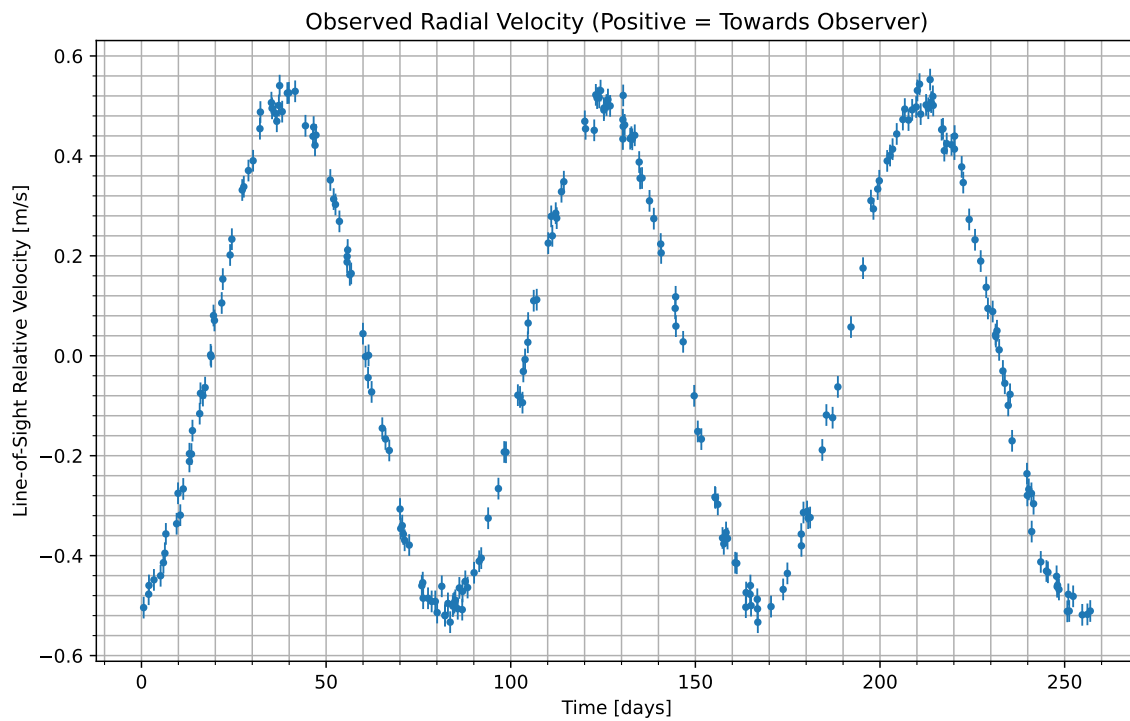
Figure 1: We have isolated the radial velocity of the host star due to the candidate planet. Data begins at UTC 2085-07-11/16:56. Positive values indicate the velocity at which the star is moving towards us; negative indicate the velocity at which it is moving away.
