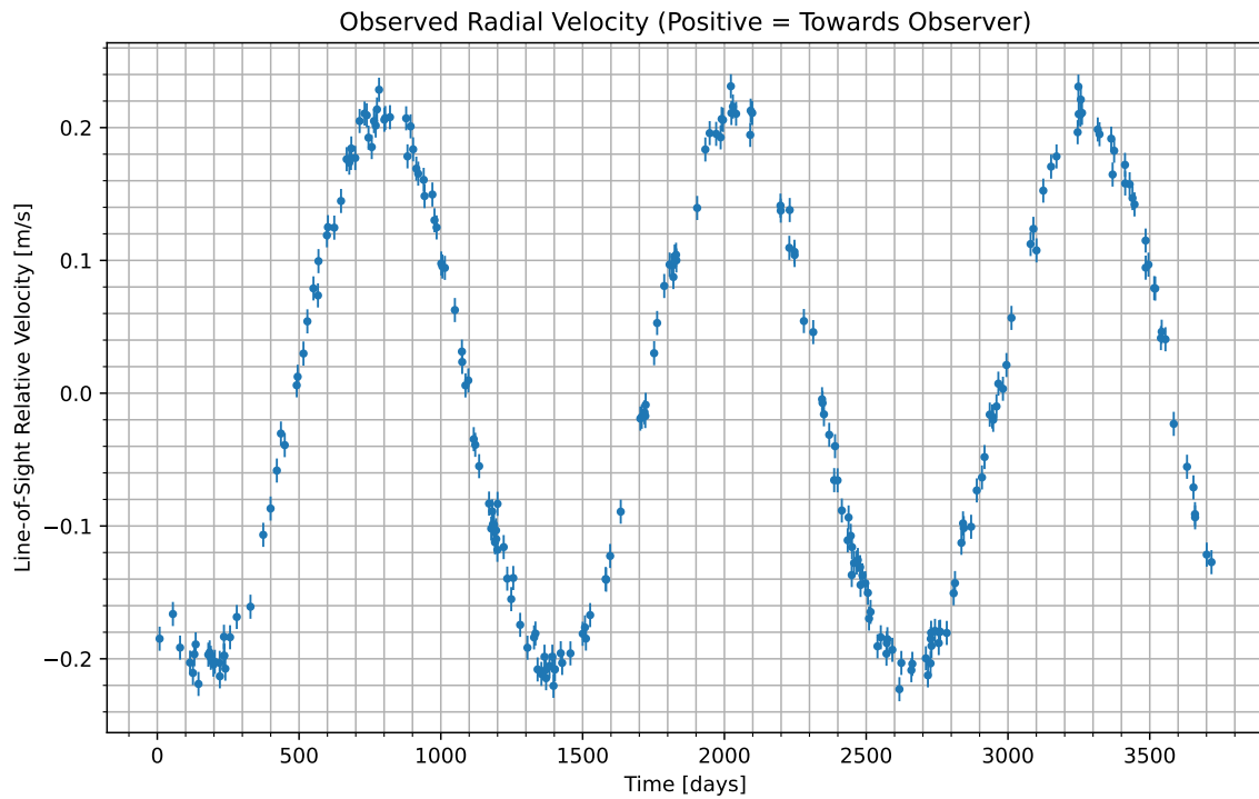
Figure 1: We have isolated the radial velocity of the host star due to the candidate planet. Data begins at UTC 2060-04-24/08:05. Positive values indicate the velocity at which the star is moving towards us; negative indicate the velocity at which it is moving away.
