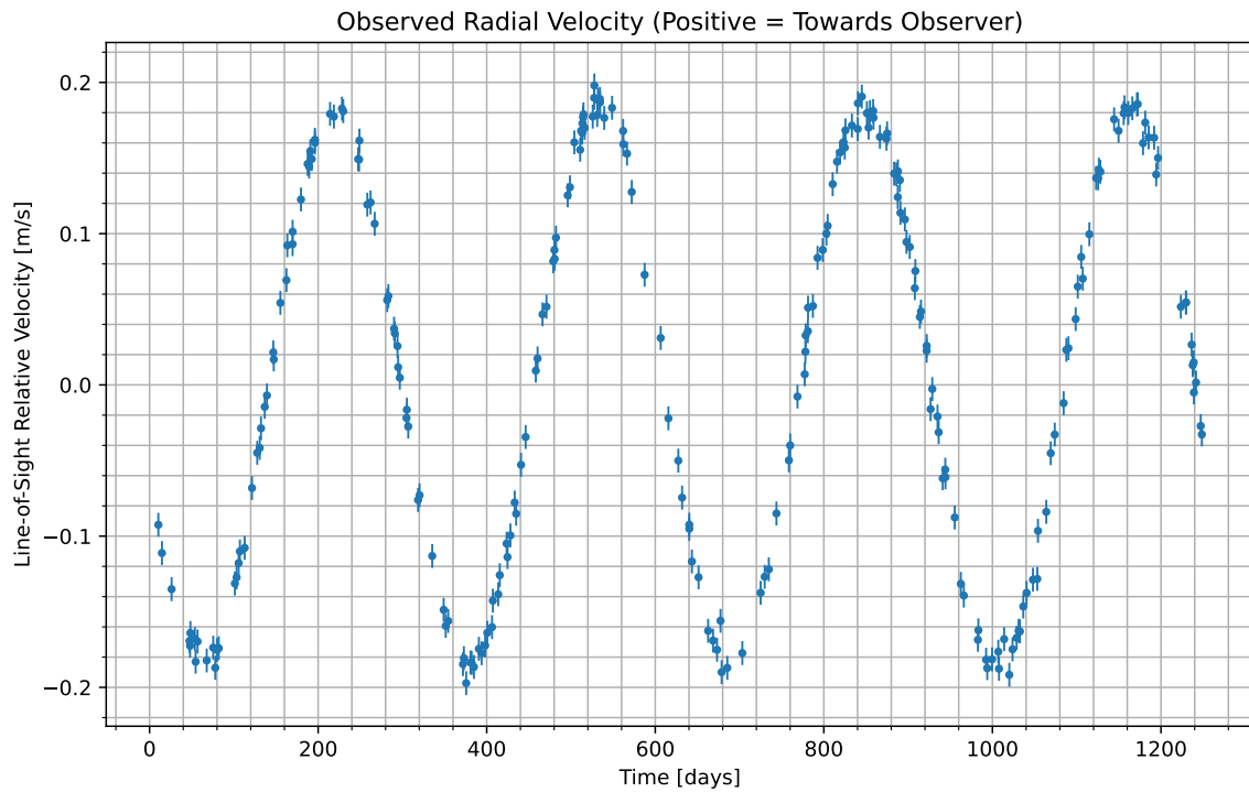
Figure 1: We have isolated the radial velocity of the host star due to the candidate planet. Data begins at UTC 2073-01-16/00:20. Positive values indicate the velocity at which the star is moving towards us; negative indicate the velocity at which it is moving away.
