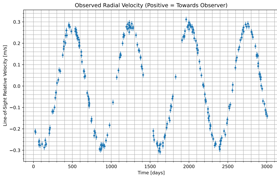
Figure 1: We have isolated the radial velocity of the host star due to the candidate planet. Data begins at UTC 2087-04-07/03:56. Positive values indicate the velocity at which the star is moving towards us; negative indicate the velocity at which it is moving away.
