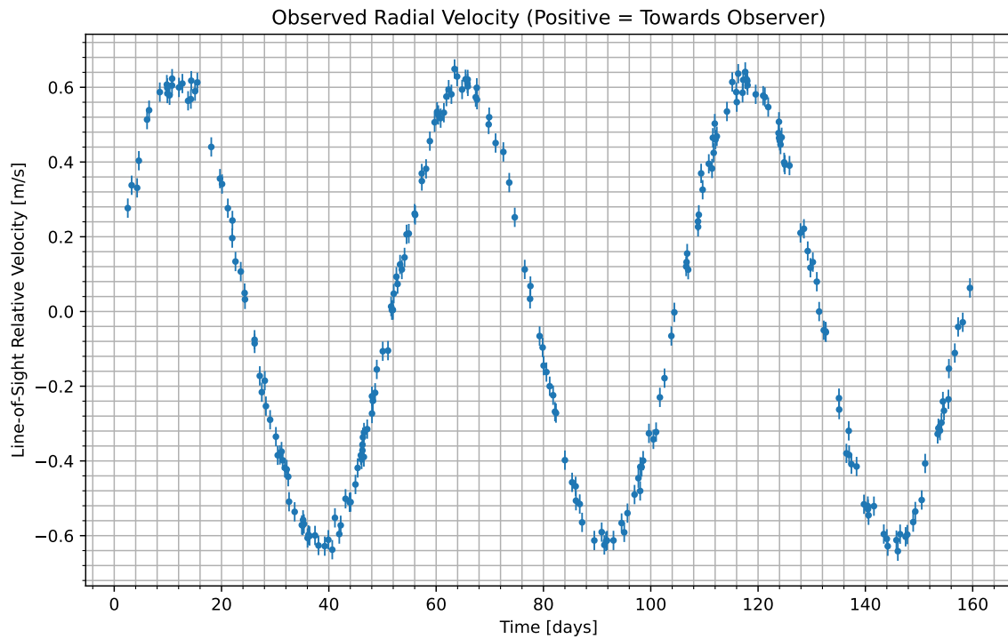
Figure 1: We have isolated the radial velocity of the host star due to the candidate planet. Data begins at UTC 2094-08-08/01:38. Positive values indicate the velocity at which the star is moving towards us; negative indicate the velocity at which it is moving away.
