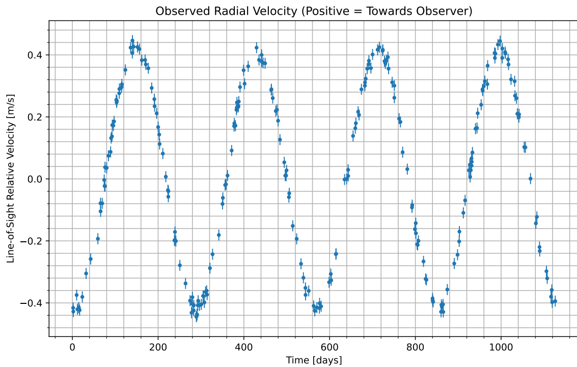
Figure 1: We have isolated the radial velocity of the host star due to the candidate planet. Data begins at UTC 2067-09-02/14:51. Positive values indicate the velocity at which the star is moving towards us; negative indicate the velocity at which it is moving away.
