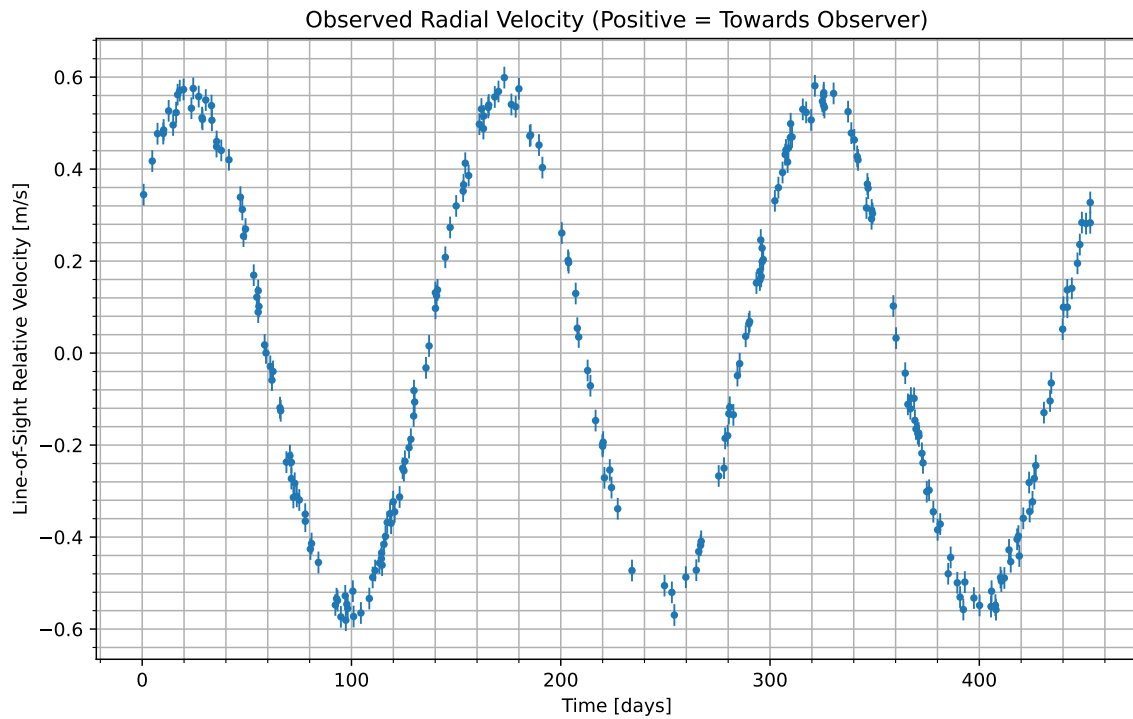
Figure 1: We have isolated the radial velocity of the host star due to the candidate planet. Data begins at UTC 2083-10-23/07:54. Positive values indicate the velocity at which the star is moving towards us; negative indicate the velocity at which it is moving away.
