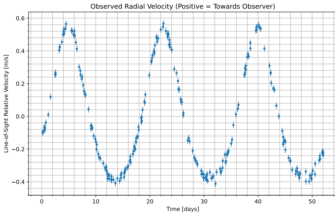
Figure 1: We have isolated the radial velocity of the host star due to the candidate planet. Data begins at UTC 2091-01-01/13:52. Positive values indicate the velocity at which the star is moving towards us; negative indicate the velocity at which it is moving away.
