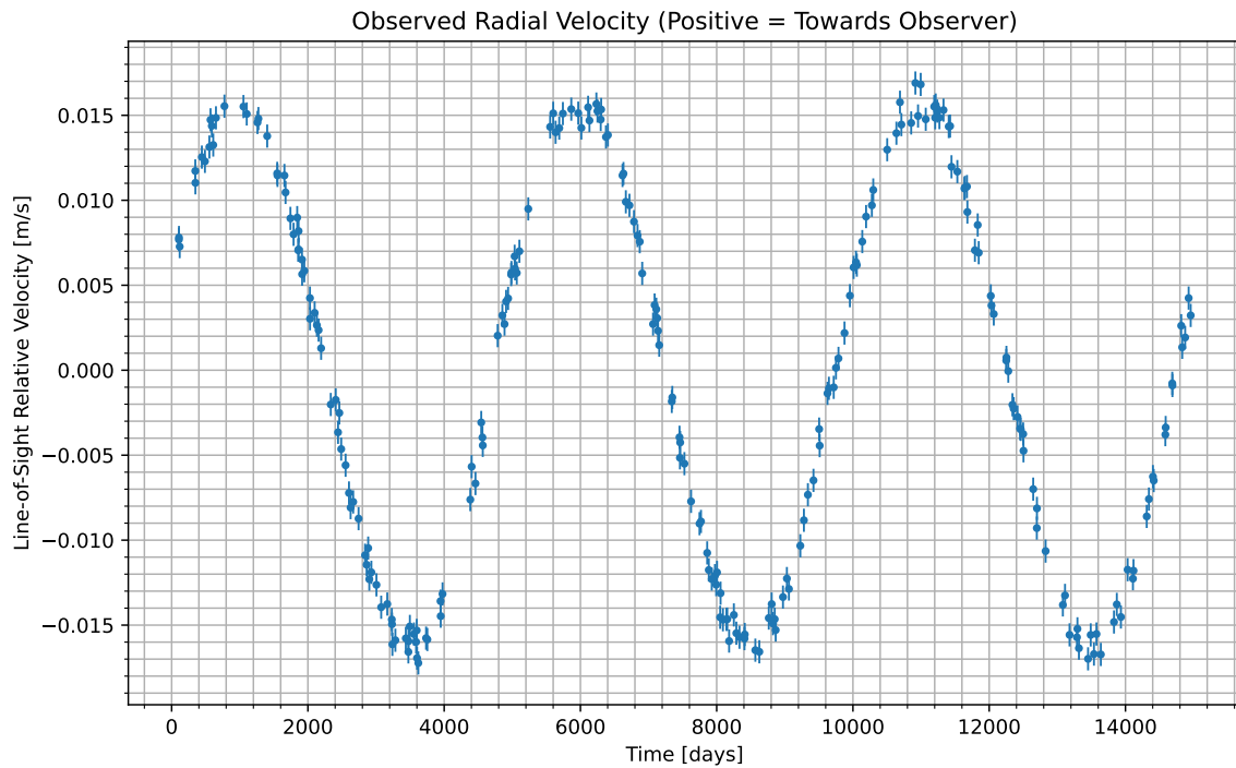
Figure 1: We have isolated the radial velocity of the host star due to the candidate planet. Data begins at UTC 2042-07-16/12:18. Positive values indicate the velocity at which the star is moving towards us; negative indicate the velocity at which it is moving away.
