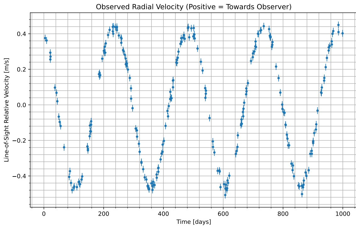
Figure 1: We have isolated the radial velocity of the host star due to the candidate planet. Data begins at UTC 2080-08-10/01:08. Positive values indicate the velocity at which the star is moving towards us; negative indicate the velocity at which it is moving away.
