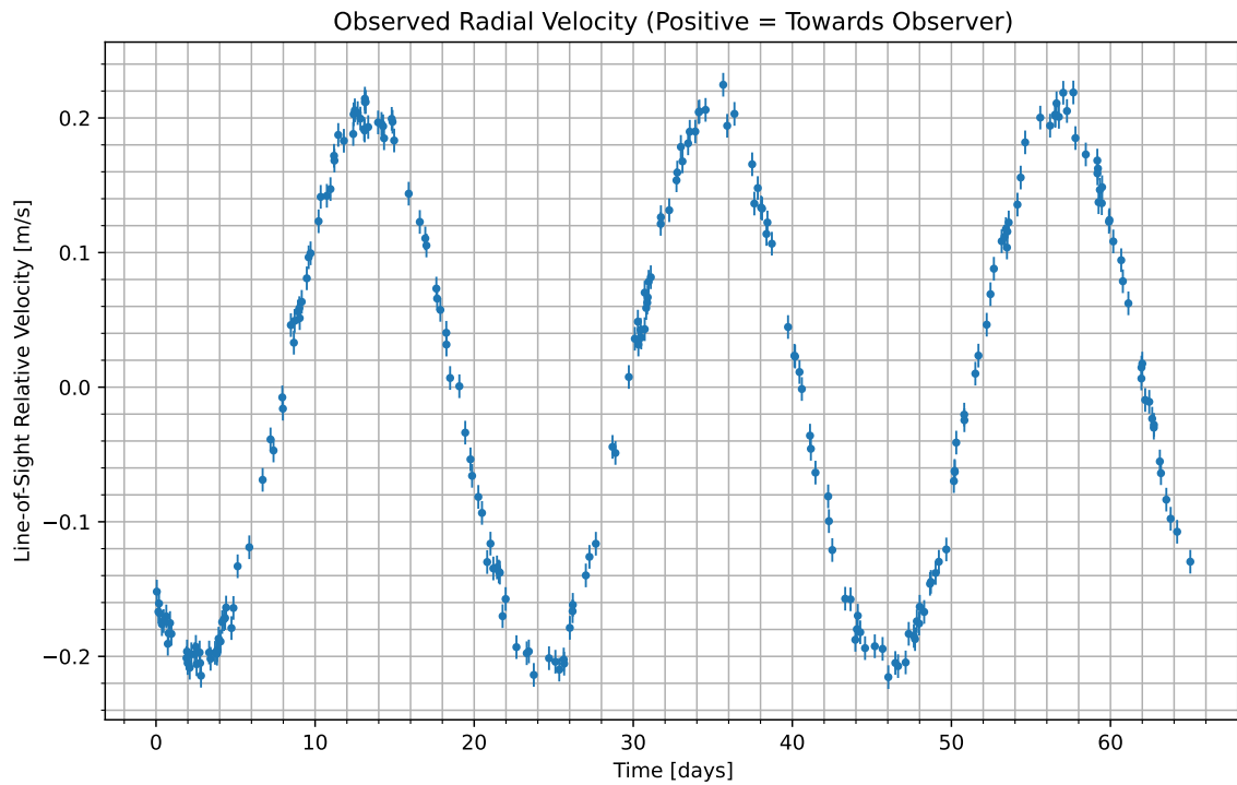
Figure 1: We have isolated the radial velocity of the host star due to the candidate planet. Data begins at UTC 2090-12-03/02:24. Positive values indicate the velocity at which the star is moving towards us; negative indicate the velocity at which it is moving away.
