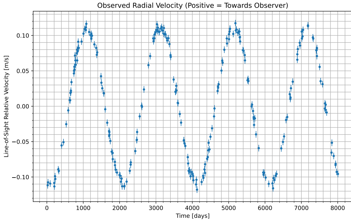
Figure 1: We have isolated the radial velocity of the host star due to the candidate planet. Data begins at UTC 2071-04-21/09:23. Positive values indicate the velocity at which the star is moving towards us; negative indicate the velocity at which it is moving away.
