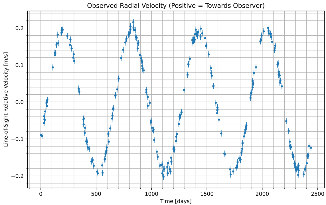
Figure 1: We have isolated the radial velocity of the host star due to the candidate planet. Data begins at UTC 2064-02-15/17:11. Positive values indicate the velocity at which the star is moving towards us; negative indicate the velocity at which it is moving away.
