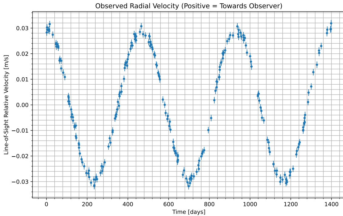
Figure 1: We have isolated the radial velocity of the host star due to the candidate planet. Data begins at UTC 2077-01-30/21:41. Positive values indicate the velocity at which the star is moving towards us; negative indicate the velocity at which it is moving away.
