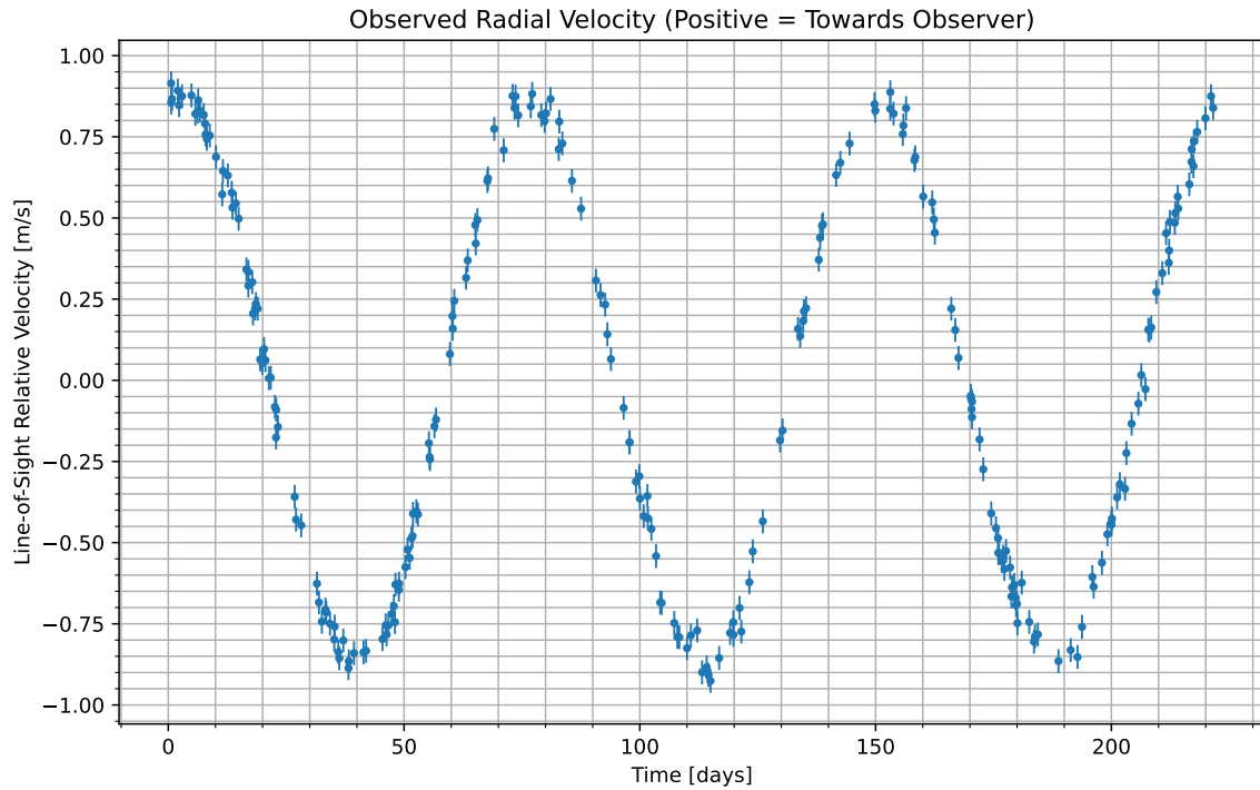
Figure 1: We have isolated the radial velocity of the host star due to the candidate planet. Data begins at UTC 2087-08-14/03:42. Positive values indicate the velocity at which the star is moving towards us; negative indicate the velocity at which it is moving away.
