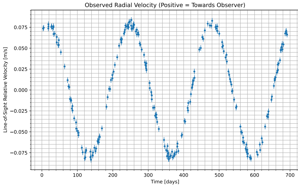
Figure 1: We have isolated the radial velocity of the host star due to the candidate planet. Data begins at UTC 2082-04-28/17:08. Positive values indicate the velocity at which the star is moving towards us; negative indicate the velocity at which it is moving away.
