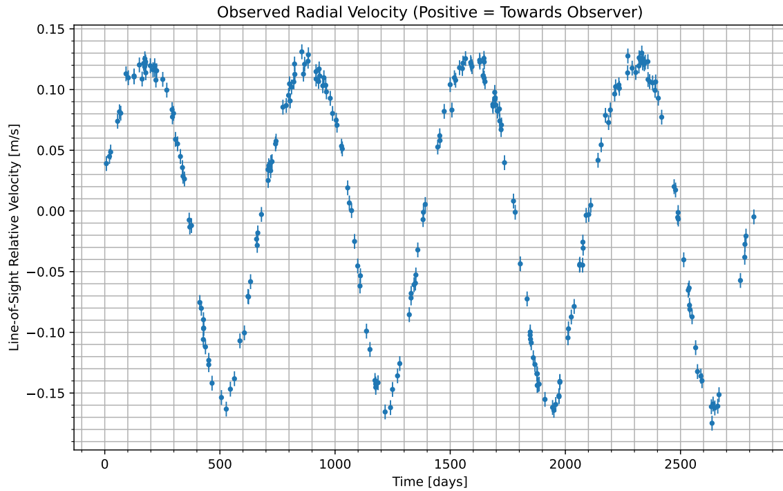
Figure 1: We have isolated the radial velocity of the host star due to the candidate planet. Data begins at UTC 2066-03-25/13:23. Positive values indicate the velocity at which the star is moving towards us; negative indicate the velocity at which it is moving away.
