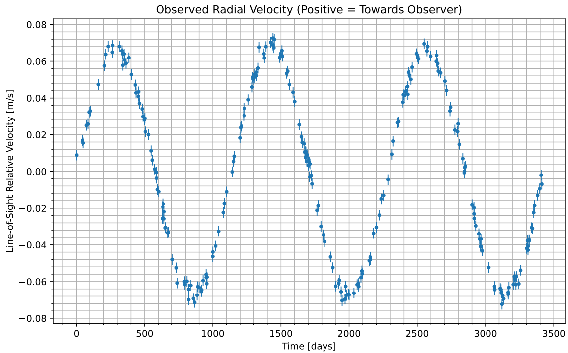
Figure 1: We have isolated the radial velocity of the host star due to the candidate planet. Data begins at UTC 2077-03-30/16:33. Positive values indicate the velocity at which the star is moving towards us; negative indicate the velocity at which it is moving away.
