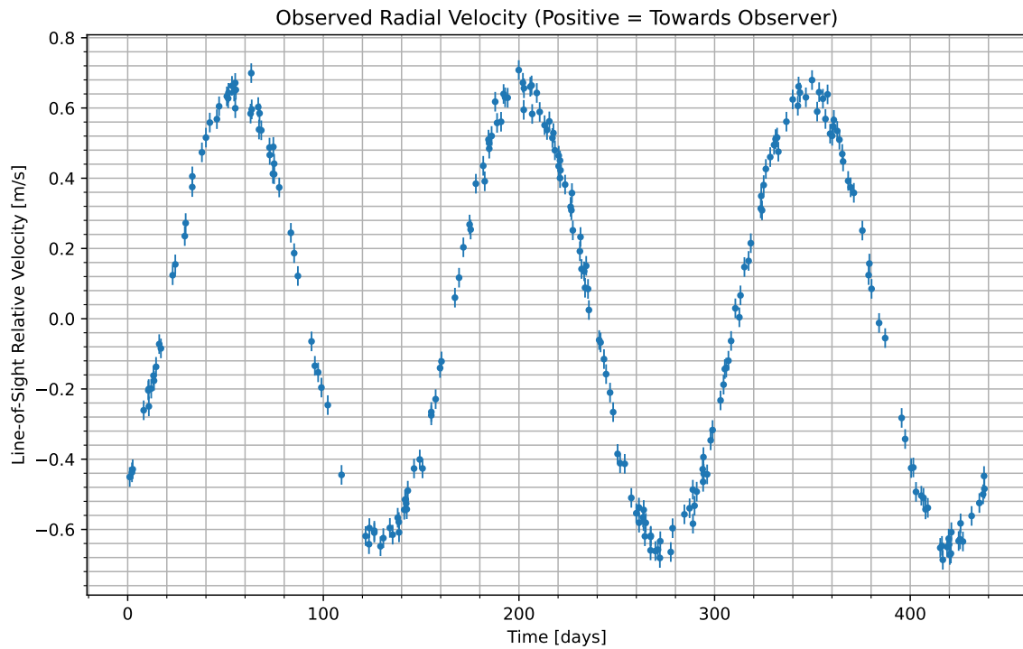
Figure 1: We have isolated the radial velocity of the host star due to the candidate planet. Data begins at UTC 2078-03-28/22:16. Positive values indicate the velocity at which the star is moving towards us; negative indicate the velocity at which it is moving away.
