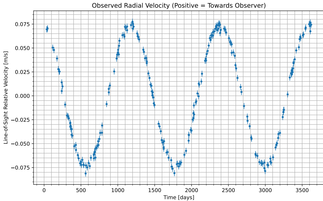
Figure 1: We have isolated the radial velocity of the host star due to the candidate planet. Data begins at UTC 2065-01-18/12:25. Positive values indicate the velocity at which the star is moving towards us; negative indicate the velocity at which it is moving away.
