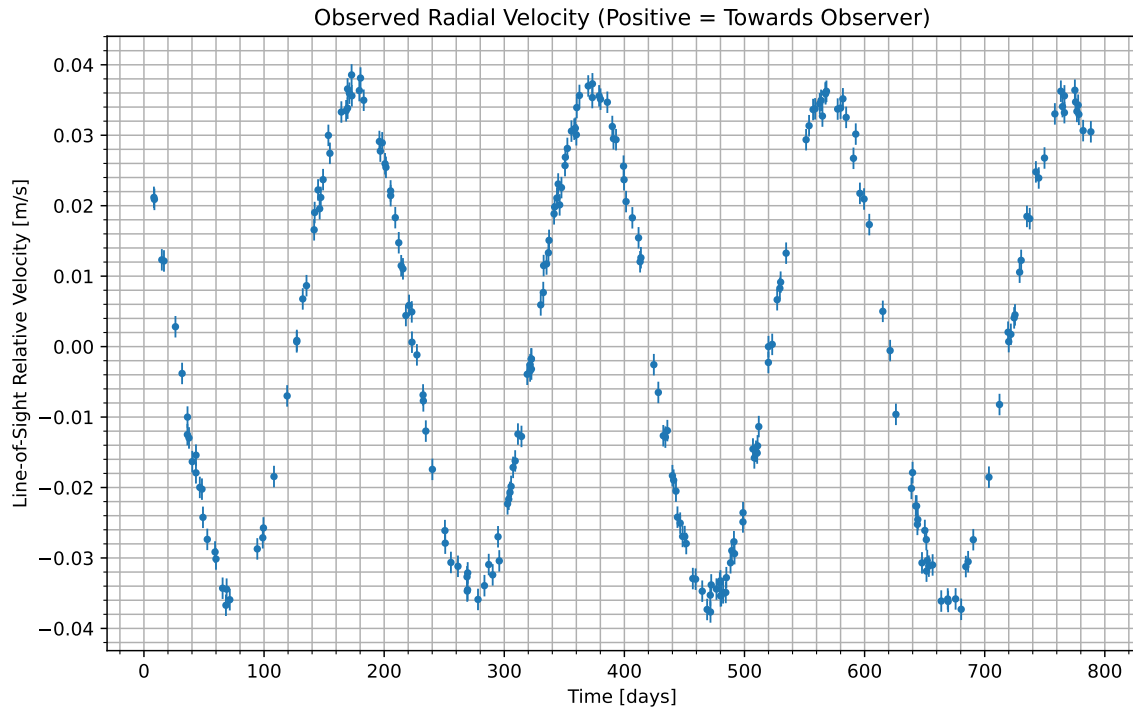
Figure 1: We have isolated the radial velocity of the host star due to the candidate planet. Data begins at UTC 2094-11-30/00:32. Positive values indicate the velocity at which the star is moving towards us; negative indicate the velocity at which it is moving away.
