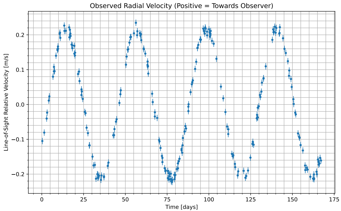
Figure 1: We have isolated the radial velocity of the host star due to the candidate planet. Data begins at UTC 2078-08-24/12:27. Positive values indicate the velocity at which the star is moving towards us; negative indicate the velocity at which it is moving away.
