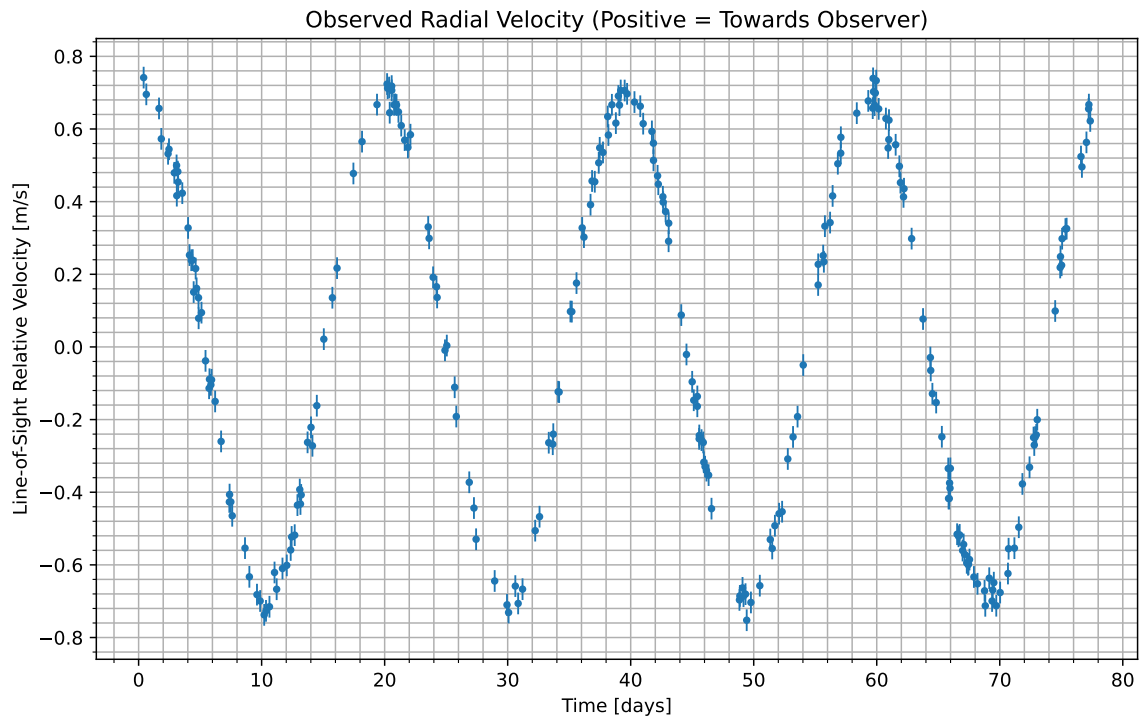
Figure 1: We have isolated the radial velocity of the host star due to the candidate planet. Data begins at UTC 2076-06-20/21:50. Positive values indicate the velocity at which the star is moving towards us; negative indicate the velocity at which it is moving away.
