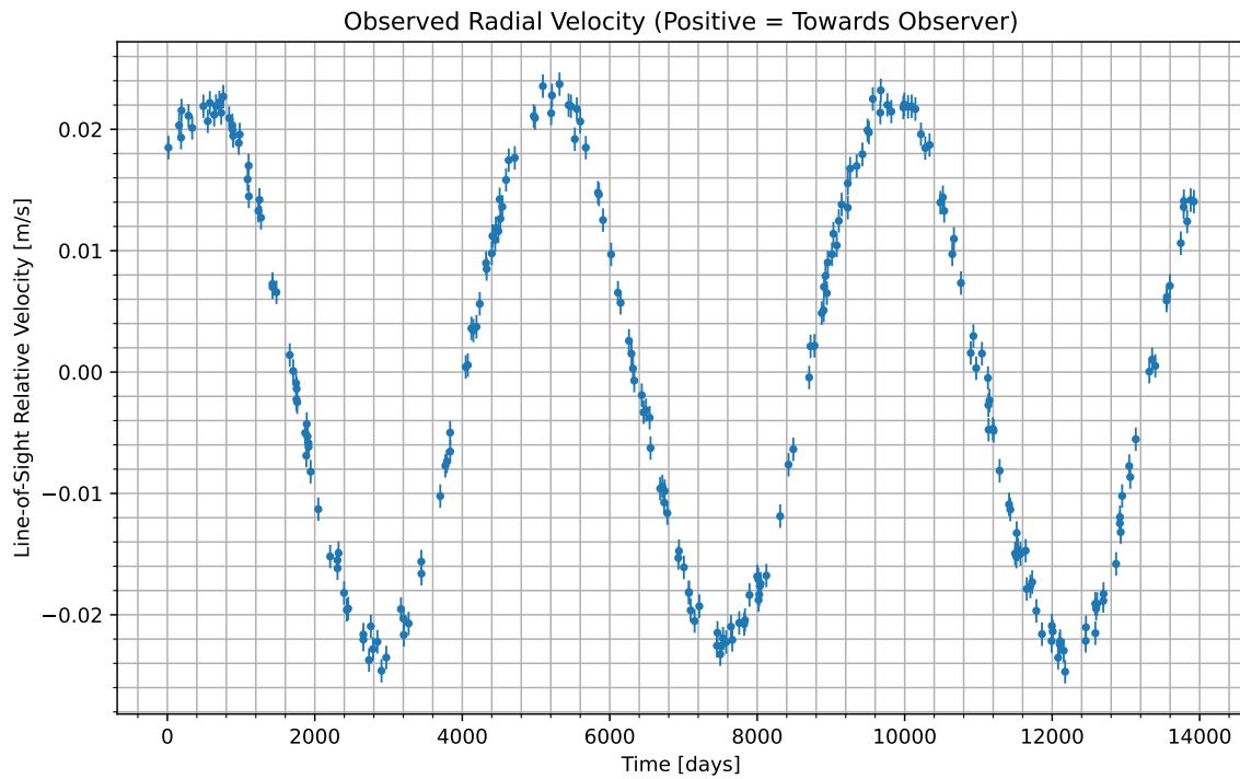
Figure 1: We have isolated the radial velocity of the host star due to the candidate planet. Data begins at UTC 2036-10-27/14:25. Positive values indicate the velocity at which the star is moving towards us; negative indicate the velocity at which it is moving away.
