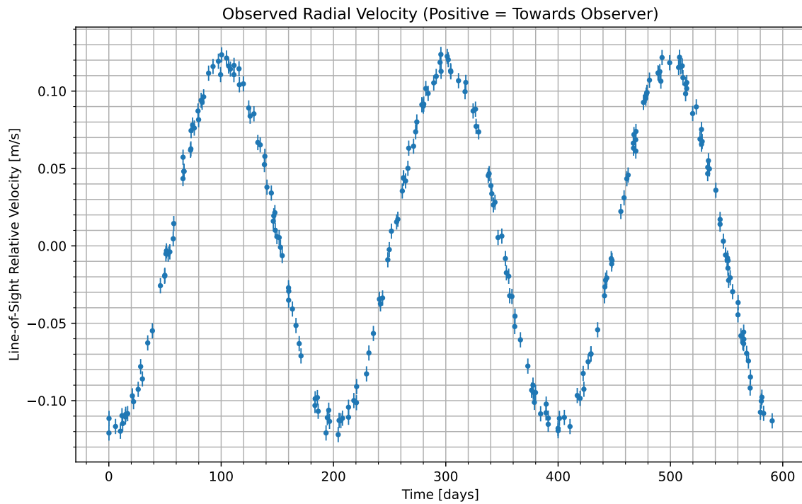
Figure 1: We have isolated the radial velocity of the host star due to the candidate planet. Data begins at UTC 2094-08-31/21:43. Positive values indicate the velocity at which the star is moving towards us; negative indicate the velocity at which it is moving away.
