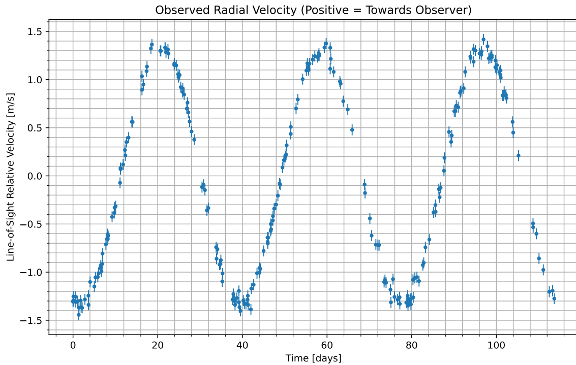
Figure 1: We have isolated the radial velocity of the host star due to the candidate planet. Data begins at UTC 2074-05-17/06:08. Positive values indicate the velocity at which the star is moving towards us; negative indicate the velocity at which it is moving away.
