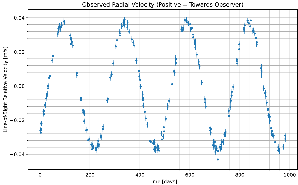
Figure 1: We have isolated the radial velocity of the host star due to the candidate planet. Data begins at UTC 2083-06-17/10:39. Positive values indicate the velocity at which the star is moving towards us; negative indicate the velocity at which it is moving away.
