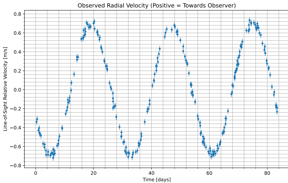
Figure 1: We have isolated the radial velocity of the host star due to the candidate planet. Data begins at UTC 2099-04-08/12:53. Positive values indicate the velocity at which the star is moving towards us; negative indicate the velocity at which it is moving away.
