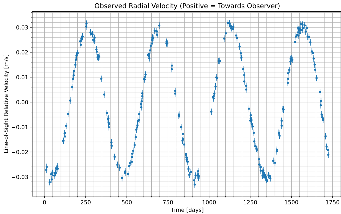
Figure 1: We have isolated the radial velocity of the host star due to the candidate planet. Data begins at UTC 2076-11-16/00:23. Positive values indicate the velocity at which the star is moving towards us; negative indicate the velocity at which it is moving away.
