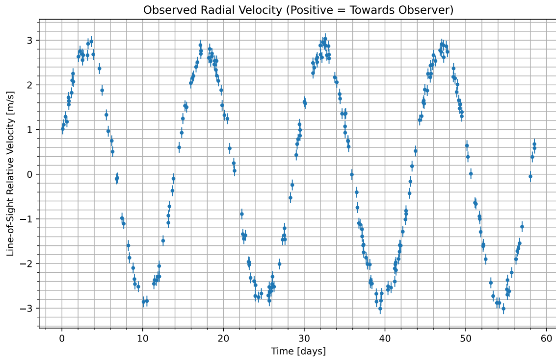
Figure 1: We have isolated the radial velocity of the host star due to the candidate planet. Data begins at UTC 2100-05-01/07:56. Positive values indicate the velocity at which the star is moving towards us; negative indicate the velocity at which it is moving away.
