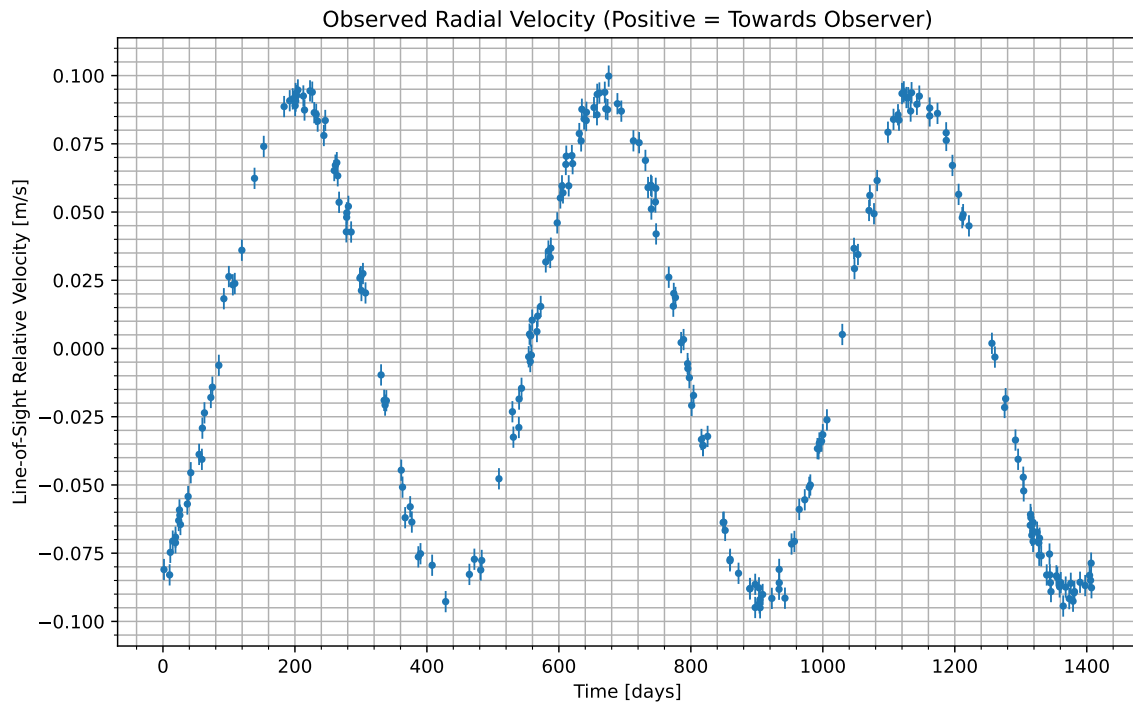
Figure 1: We have isolated the radial velocity of the host star due to the candidate planet. Data begins at UTC 2079-09-04/21:31. Positive values indicate the velocity at which the star is moving towards us; negative indicate the velocity at which it is moving away.
