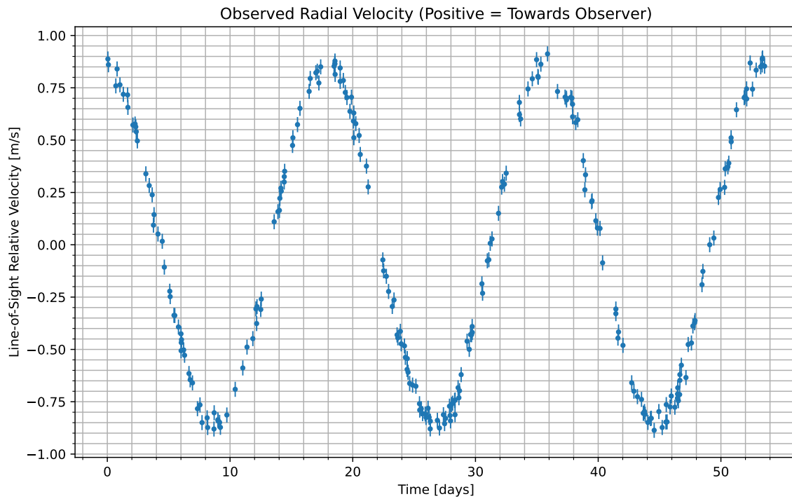
Figure 1: We have isolated the radial velocity of the host star due to the candidate planet. Data begins at UTC 2072-11-13/19:52. Positive values indicate the velocity at which the star is moving towards us; negative indicate the velocity at which it is moving away.
