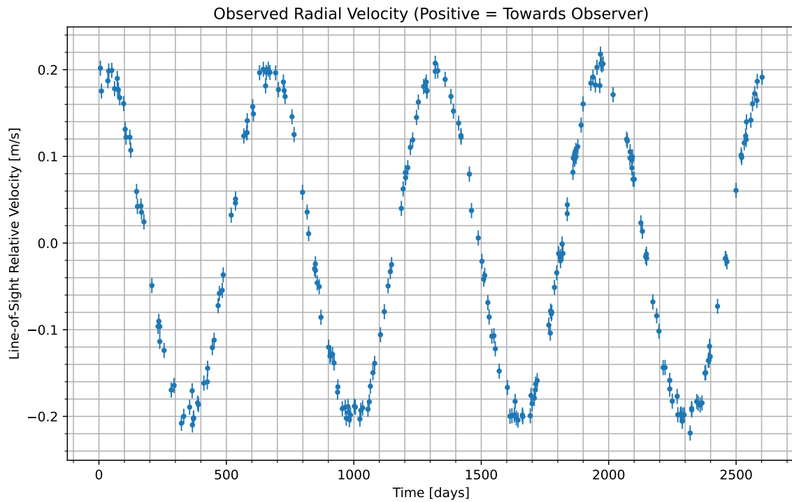
Figure 1: We have isolated the radial velocity of the host star due to the candidate planet. Data begins at UTC 2065-11-25/09:57. Positive values indicate the velocity at which the star is moving towards us; negative indicate the velocity at which it is moving away.
