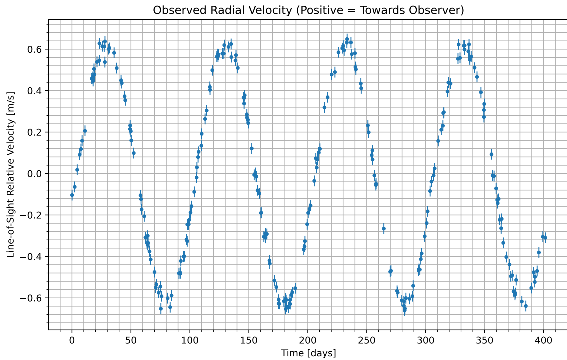
Figure 1: We have isolated the radial velocity of the host star due to the candidate planet. Data begins at UTC 2079-12-19/09:15. Positive values indicate the velocity at which the star is moving towards us; negative indicate the velocity at which it is moving away.
