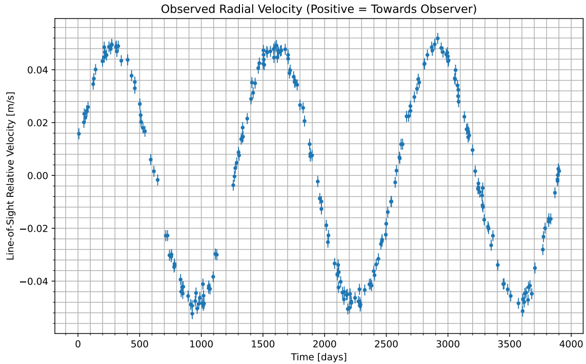
Figure 1: We have isolated the radial velocity of the host star due to the candidate planet. Data begins at UTC 2061-10-21/08:27. Positive values indicate the velocity at which the star is moving towards us; negative indicate the velocity at which it is moving away.
