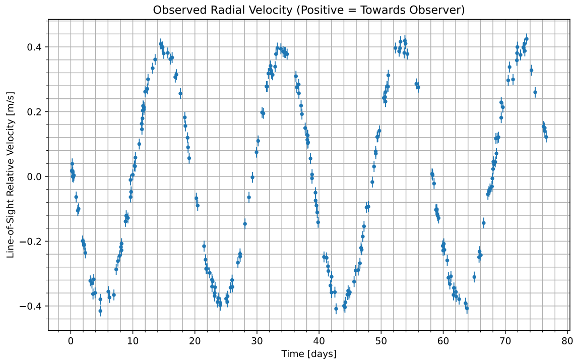
Figure 1: We have isolated the radial velocity of the host star due to the candidate planet. Data begins at UTC 2077-11-24/17:51. Positive values indicate the velocity at which the star is moving towards us; negative indicate the velocity at which it is moving away.
