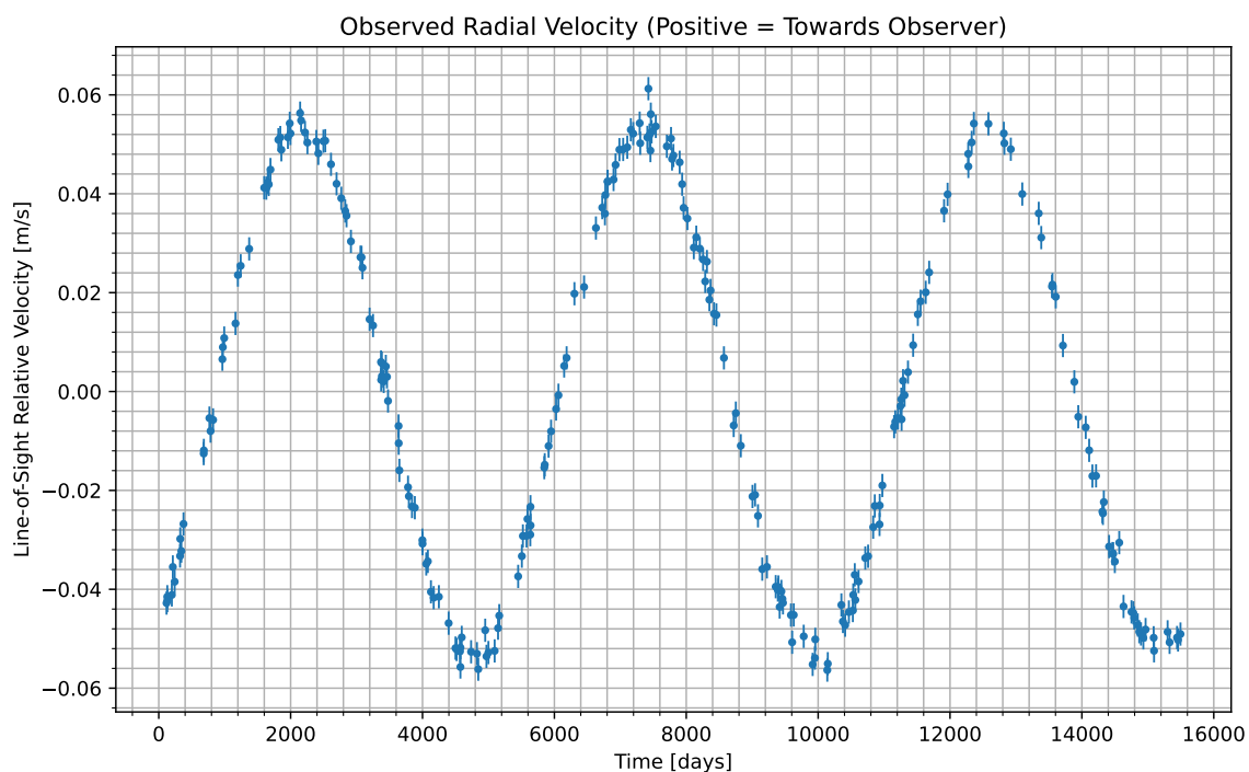
Figure 1: We have isolated the radial velocity of the host star due to the candidate planet. Data begins at UTC 2051-07-26/11:21. Positive values indicate the velocity at which the star is moving towards us; negative indicate the velocity at which it is moving away.
