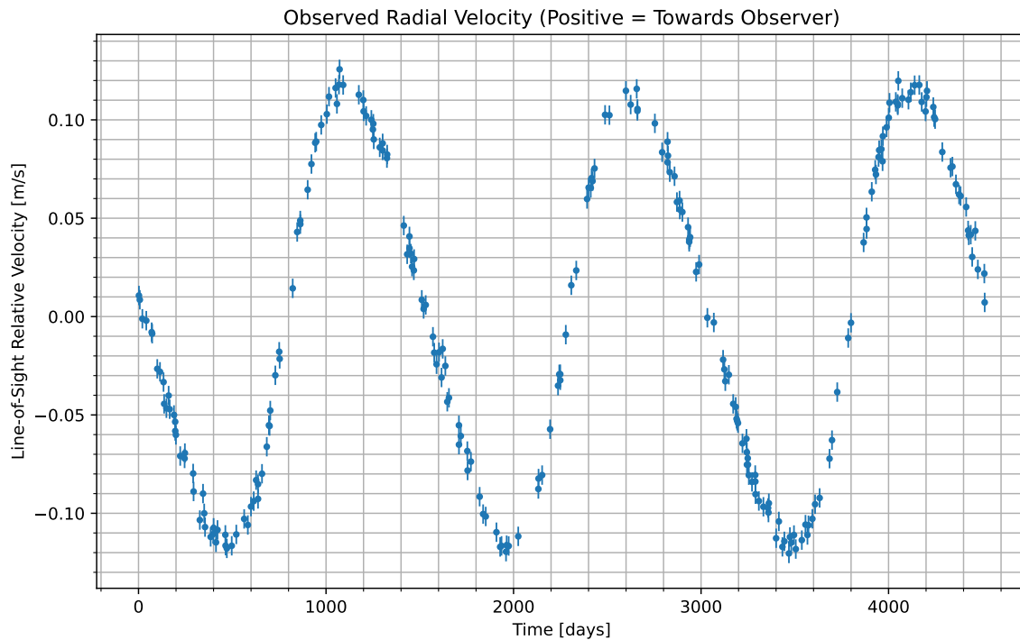
Figure 1: We have isolated the radial velocity of the host star due to the candidate planet. Data begins at UTC 2070-10-13/21:21. Positive values indicate the velocity at which the star is moving towards us; negative indicate the velocity at which it is moving away.
