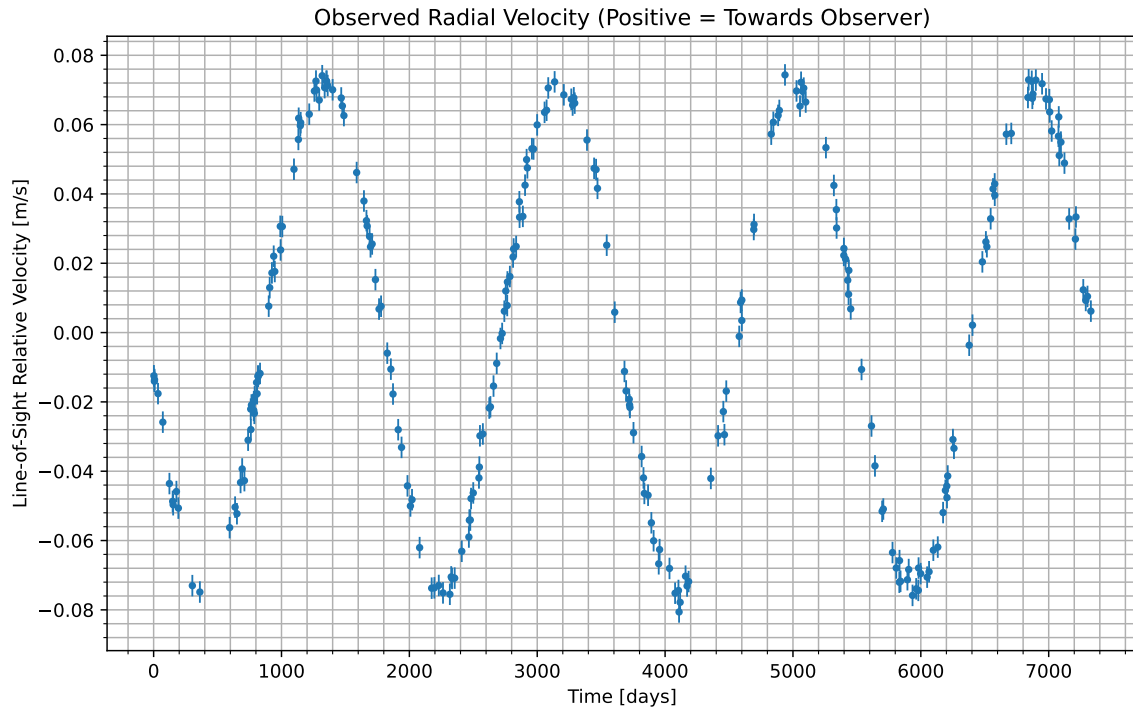
Figure 1: We have isolated the radial velocity of the host star due to the candidate planet. Data begins at UTC 2053-02-22/22:27. Positive values indicate the velocity at which the star is moving towards us; negative indicate the velocity at which it is moving away.
