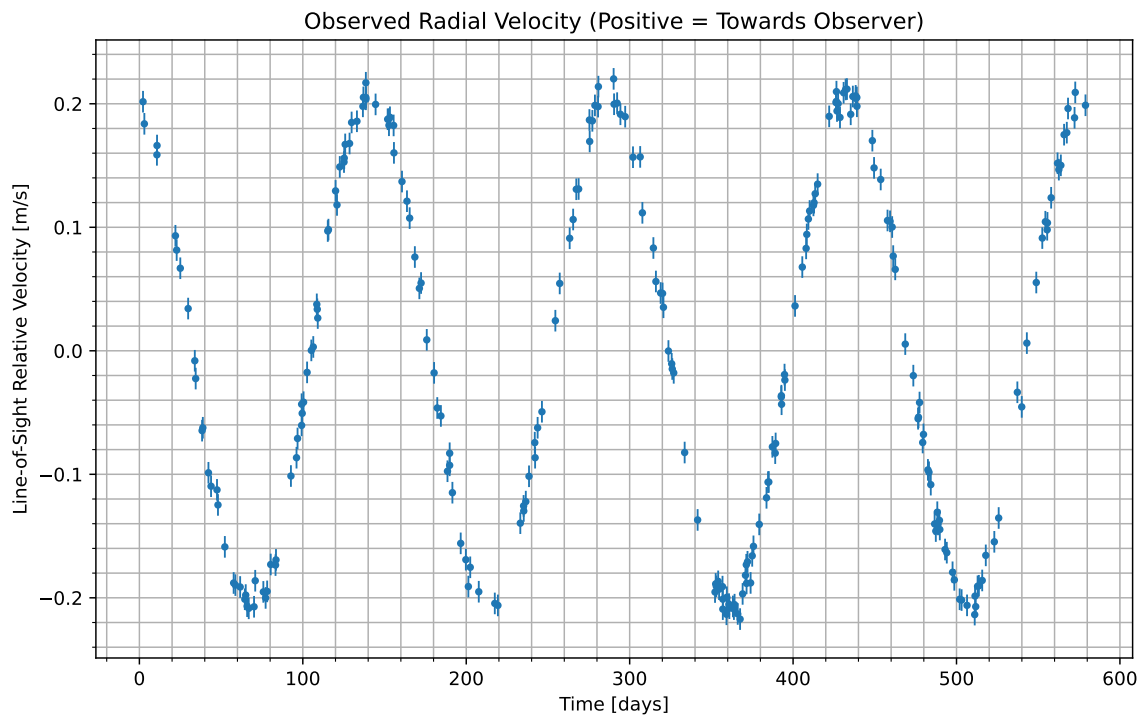
Figure 1: We have isolated the radial velocity of the host star due to the candidate planet. Data begins at UTC 2072-04-04/22:57. Positive values indicate the velocity at which the star is moving towards us; negative indicate the velocity at which it is moving away.
