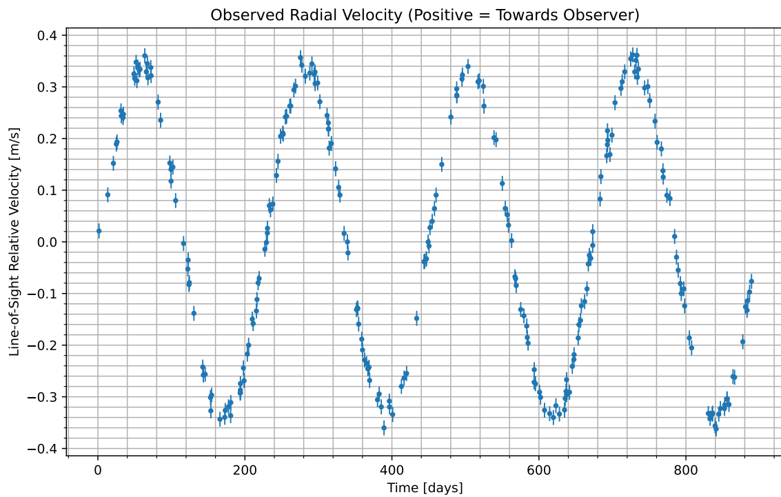
Figure 1: We have isolated the radial velocity of the host star due to the candidate planet. Data begins at UTC 2074-09-10/17:48. Positive values indicate the velocity at which the star is moving towards us; negative indicate the velocity at which it is moving away.
