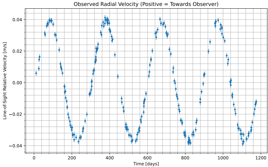
Figure 1: We have isolated the radial velocity of the host star due to the candidate planet. Data begins at UTC 2080-05-15/10:24. Positive values indicate the velocity at which the star is moving towards us; negative indicate the velocity at which it is moving away.
