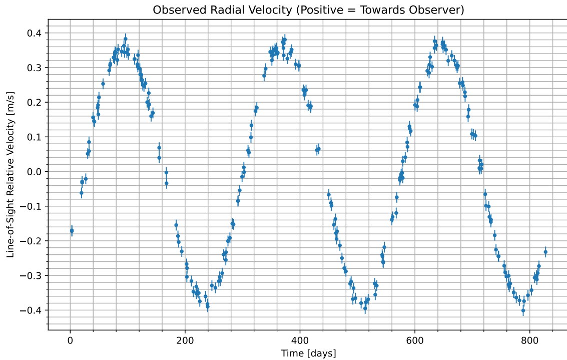
Figure 1: We have isolated the radial velocity of the host star due to the candidate planet. Data begins at UTC 2087-01-25/14:02. Positive values indicate the velocity at which the star is moving towards us; negative indicate the velocity at which it is moving away.
