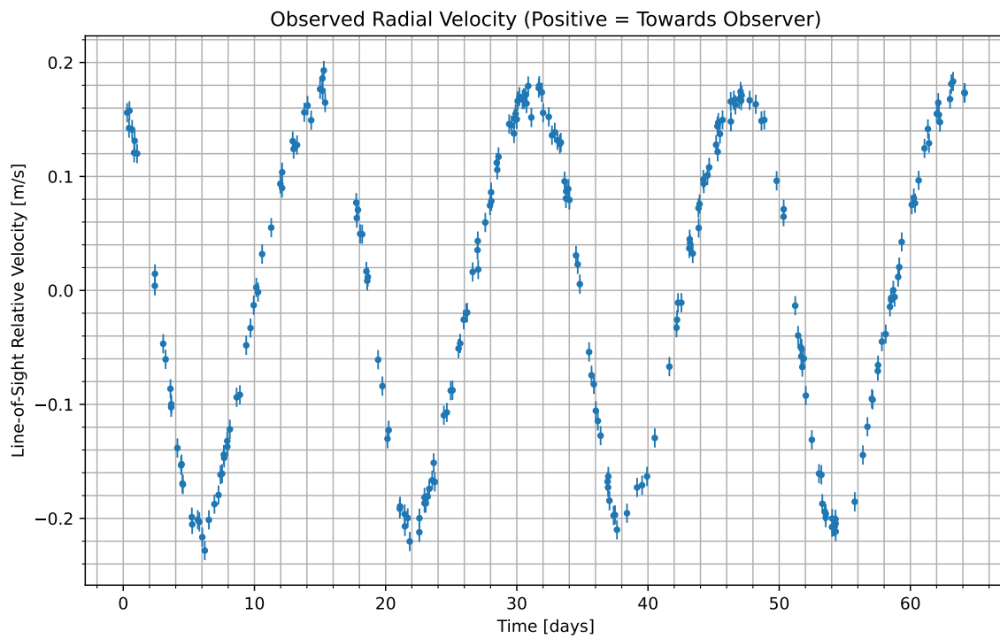
Figure 1: We have isolated the radial velocity of the host star due to the candidate planet. Data begins at UTC 2093-07-05/02:49. Positive values indicate the velocity at which the star is moving towards us; negative indicate the velocity at which it is moving away.
