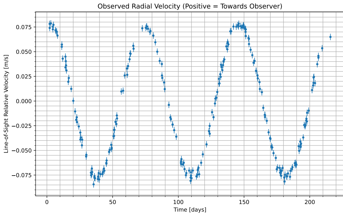
Figure 1: We have isolated the radial velocity of the host star due to the candidate planet. Data begins at UTC 2074-04-13/16:52. Positive values indicate the velocity at which the star is moving towards us; negative indicate the velocity at which it is moving away.
